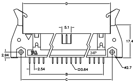
Straight Type
